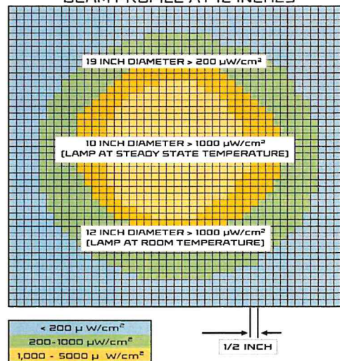
BEAM PROFILE AT 12 INCHES
